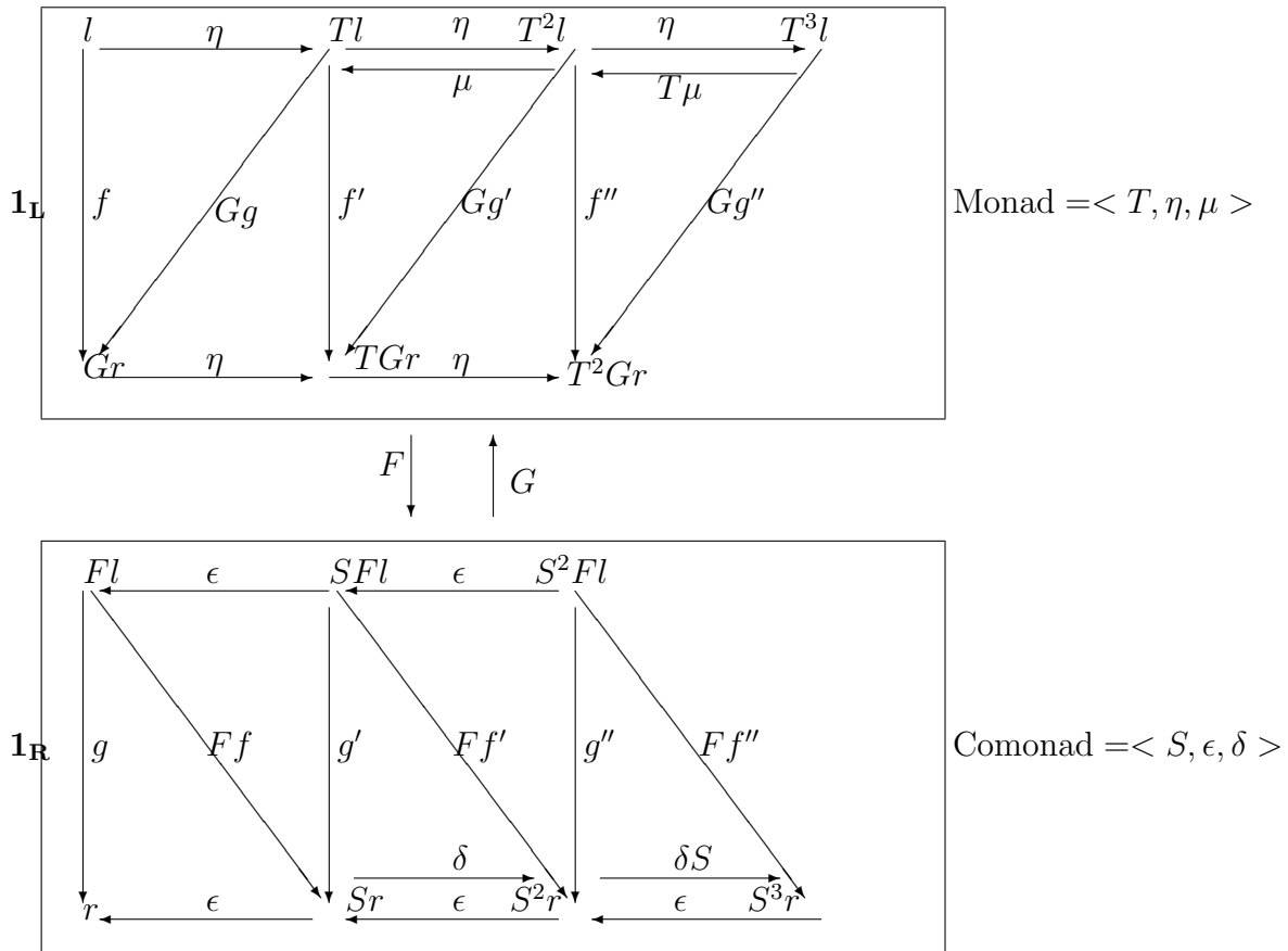
Figure 2: After three cycles GFGFGF from left-hand category and three cycles FGFGFG from right-hand category: \eta and \delta map onto other than \perp , \top maps onto other than \epsilon and \mu
